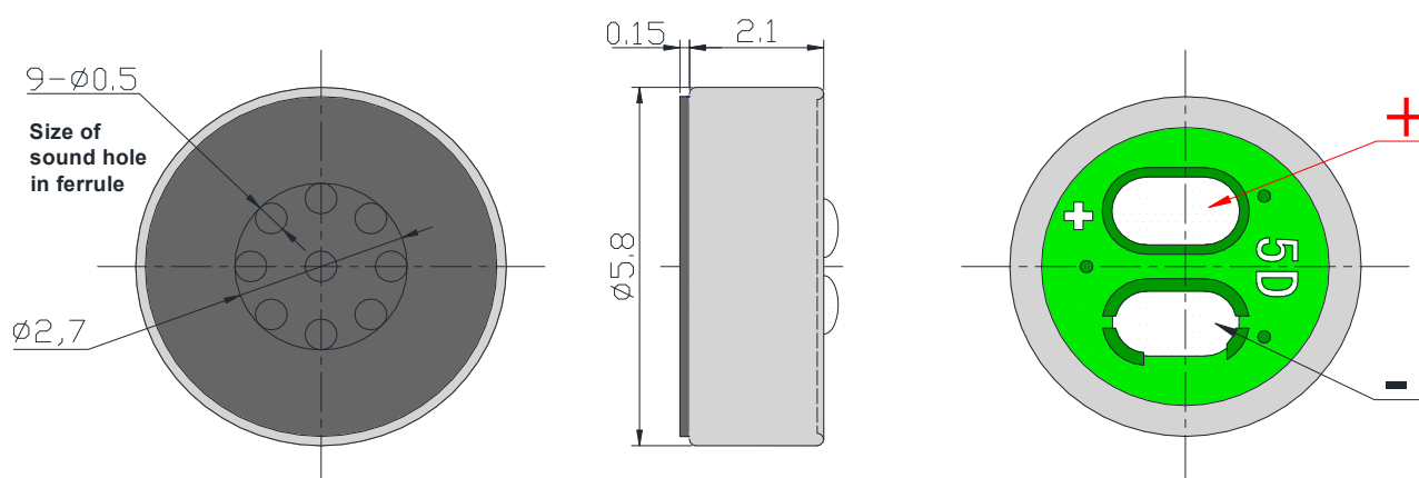
Fig. 7-1 Microphone Capsule
