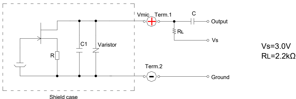
Fig. 5-1 Schematic Diagram
