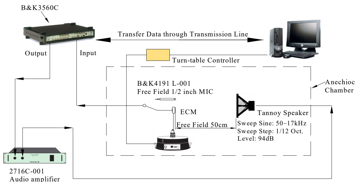
Fig. 6-1 Measurement System Setup
