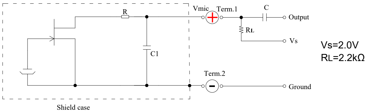
Fig. 5-1 Schematic Diagram
