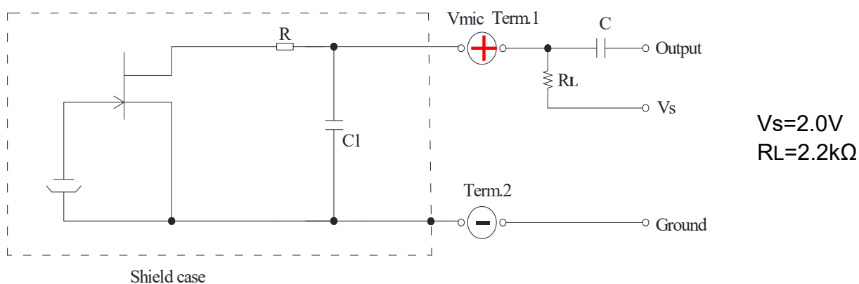
Fig. 5-1 Schematic Diagram
