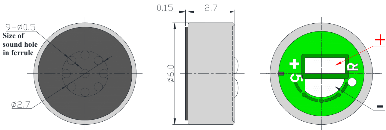
Fig. 7-1 Microphone Capsule
