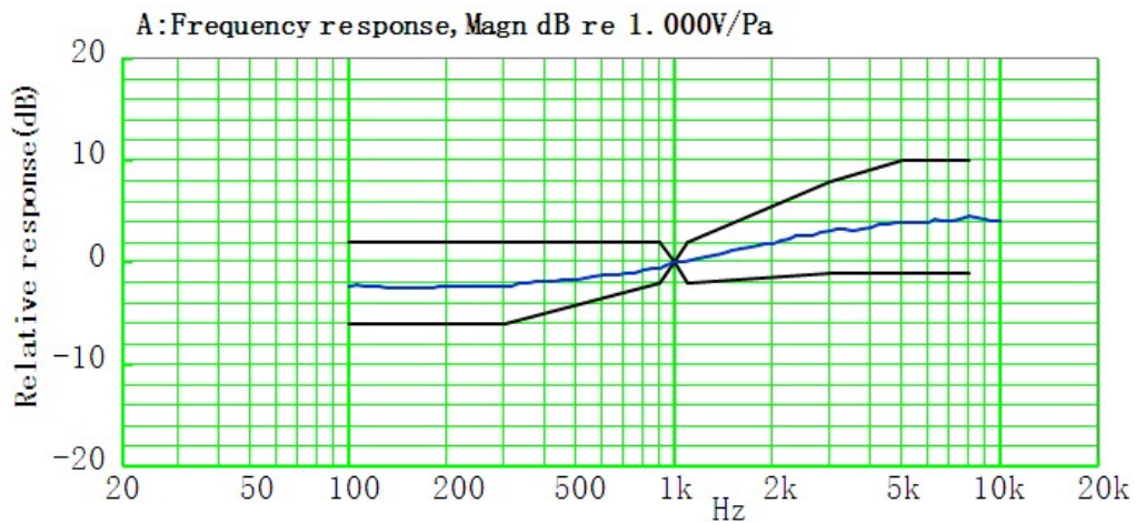
Fig. 4-1 Typical Frequency Response
