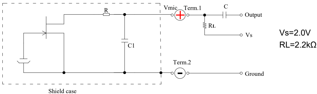
Fig. 5-1 Schematic Diagram
