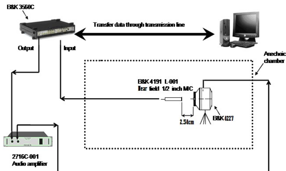
Fig. 6-1 Measurement System Setup
