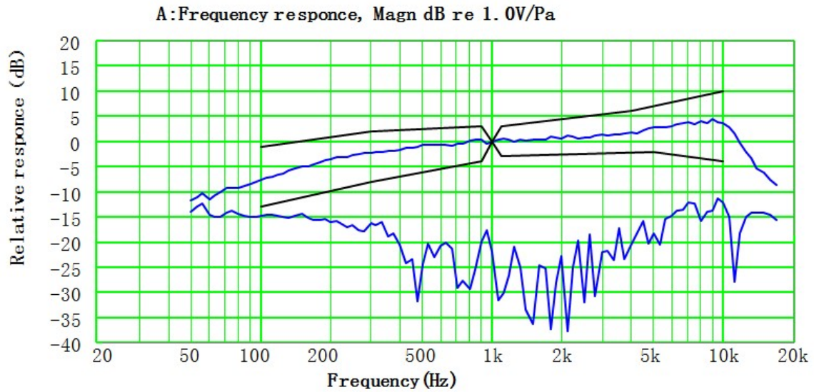
Fig. 4-1 Typical Frequency Response
