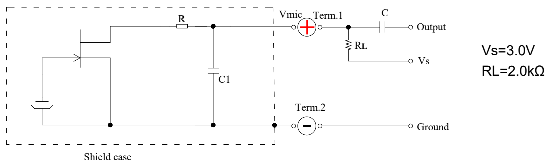
Fig. 5-1 Schematic Diagram
