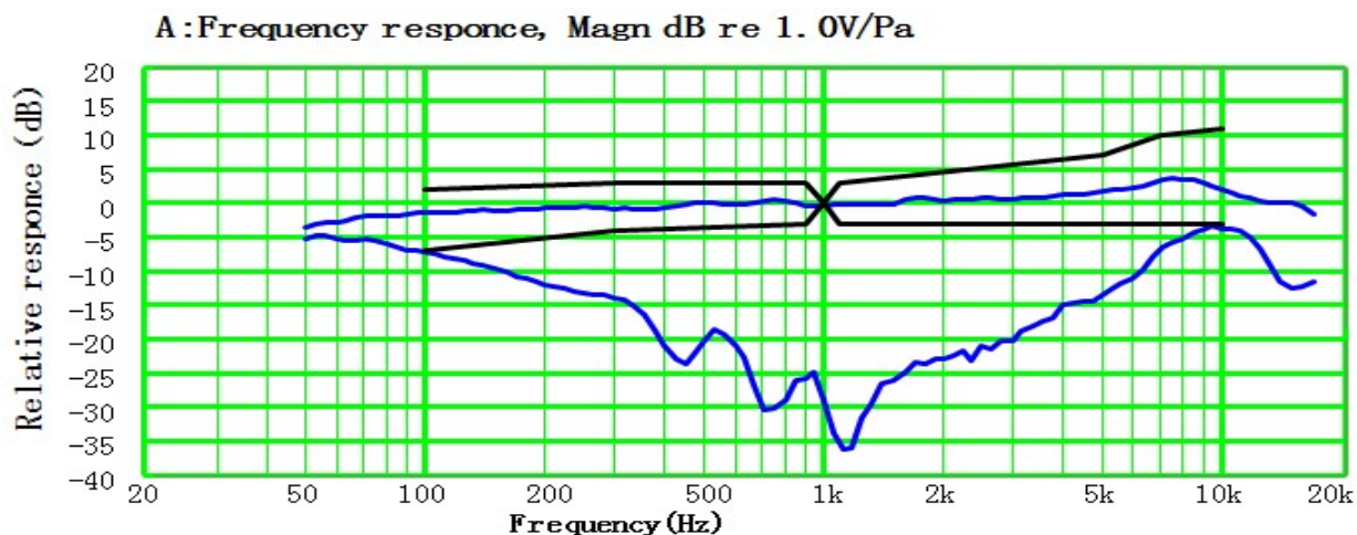
Fig. 4-1 Typical Frequency Response
