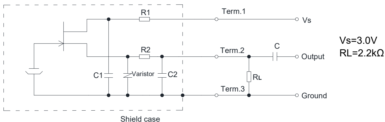
Fig. 5-1 Schematic Diagram
