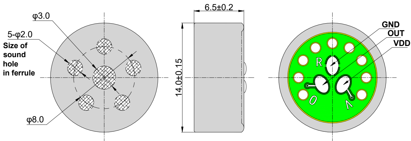
Fig. 7-1 Microphone Capsule
