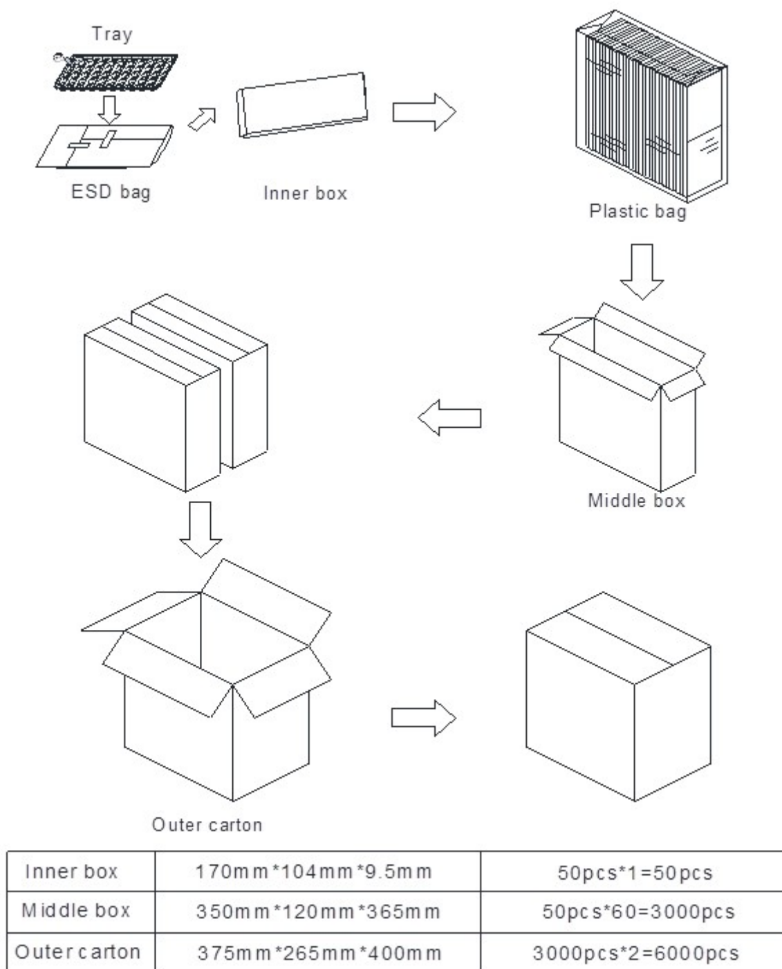
Fig. 9-1 Packaging
