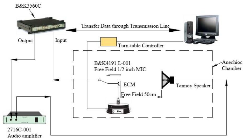
Fig. 6-1 Measurement System Setup
