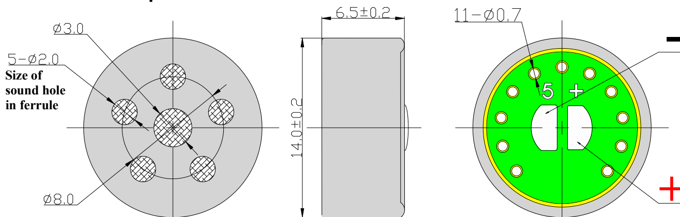
Fig. 7-1 Microphone Capsule
