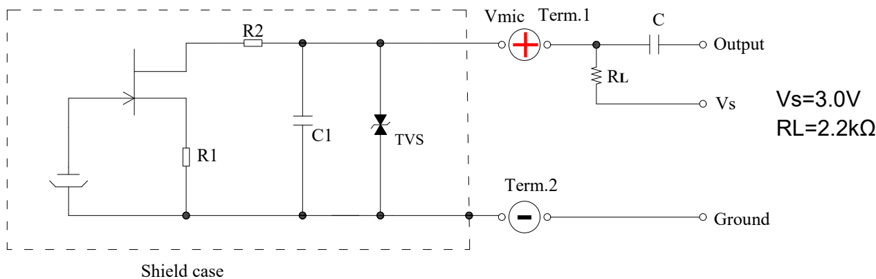
Fig. 5-1 Schematic Diagram
