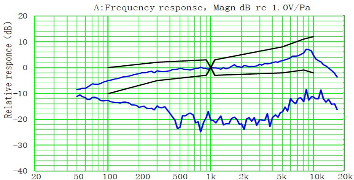
Fig. 4-1 Typical Frequency Response
