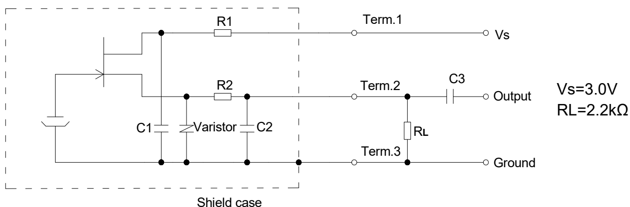
Fig. 5-1 Schematic Diagram
