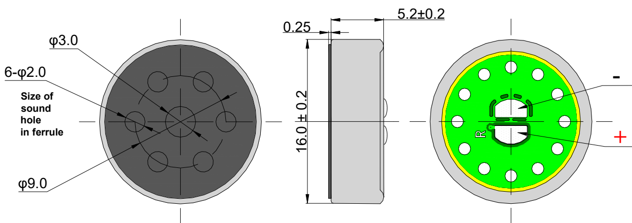
Fig. 7-1 Microphone Capsule
