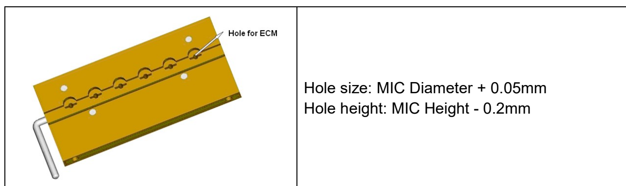
Fig. 10-1 Soldering Fixture
