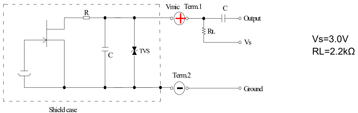
Fig. 5-1 Schematic Diagram
