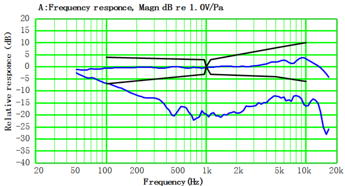
Fig. 4-1 Typical Frequency Response
