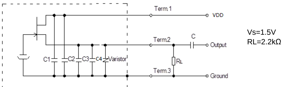
Fig. 5-1 Schematic Diagram
