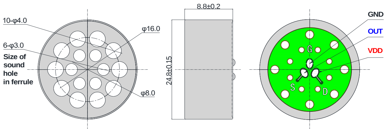
Fig. 7-1 Microphone Capsule
