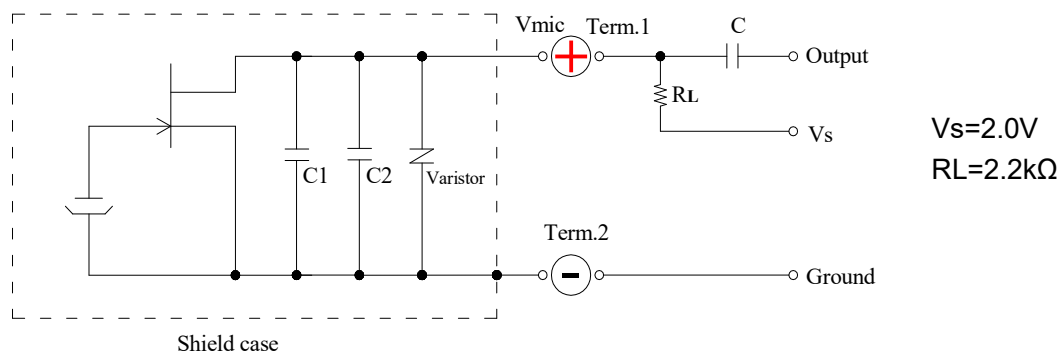
Fig. 5-1 Schematic Diagram
