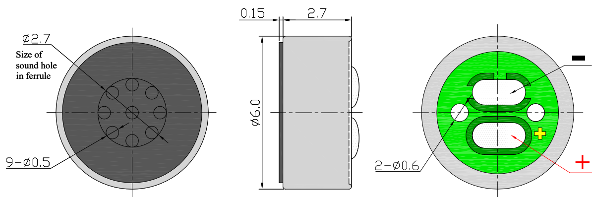
Fig. 7-1 Microphone Capsule
