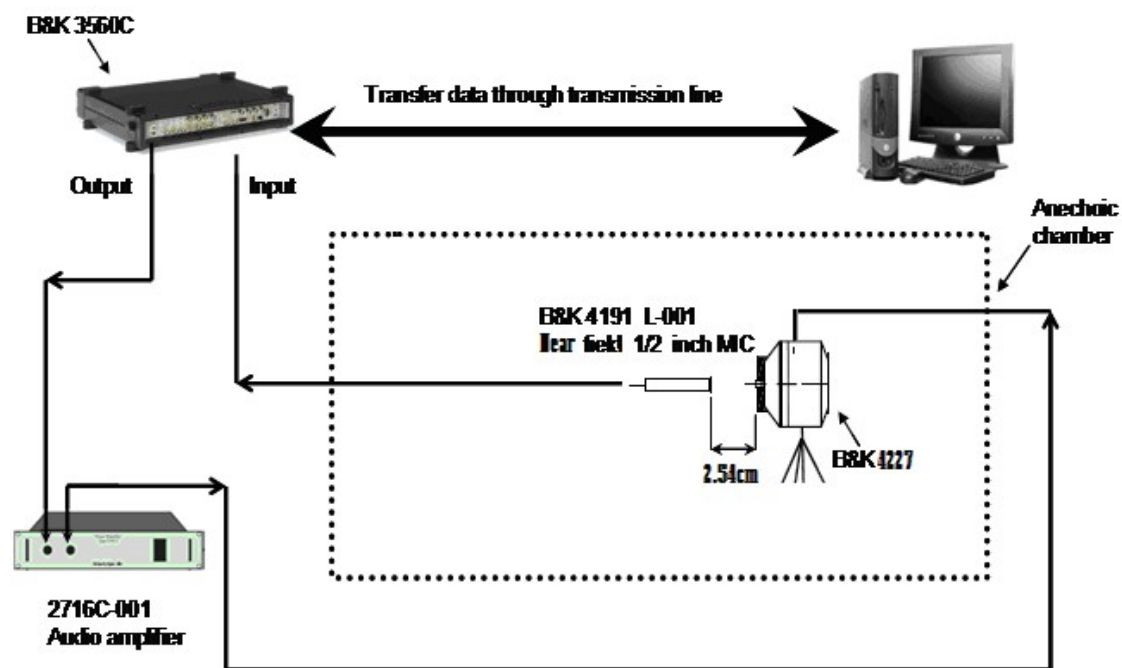
Fig. 6-1 Measurement System Setup
