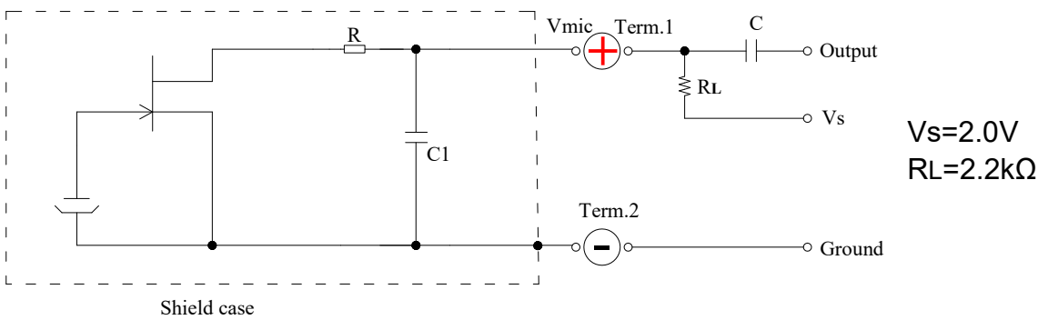
Fig. 5-1 Schematic Diagram
