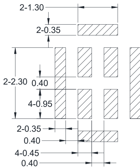
Example Land Pattern
