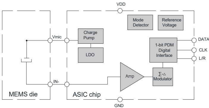
Fig. 1 Microphone block diagram
