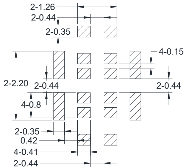
Example Solder Stencil Pattern
