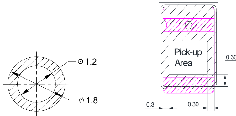
Fig. 16 Recommended nozzle for reflow MIC and Pick-up Area
