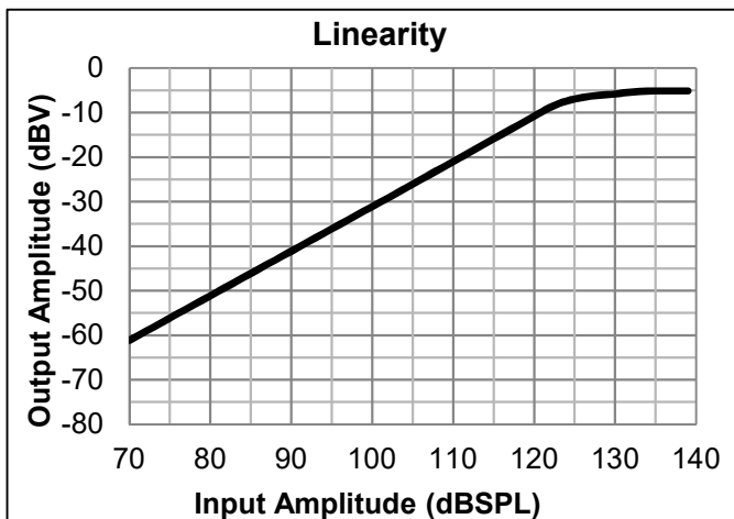
Fig. 6 Linearity
