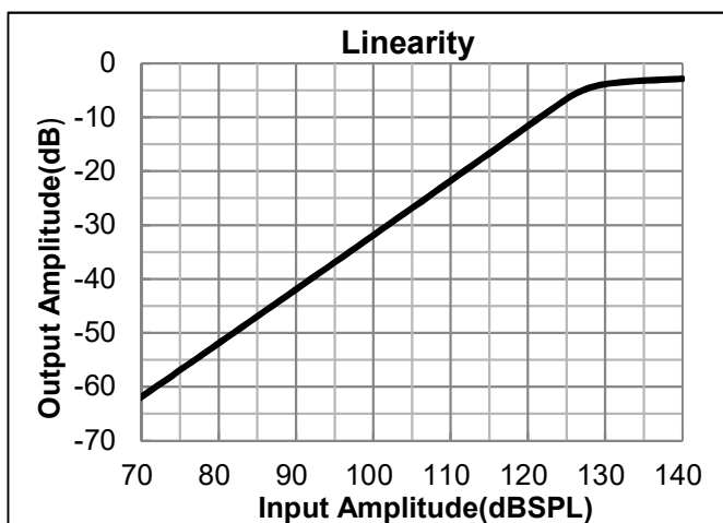
Fig. 6 Linearity
