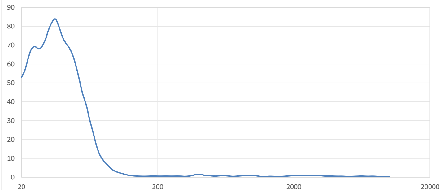
4寸全频-1W/1m
