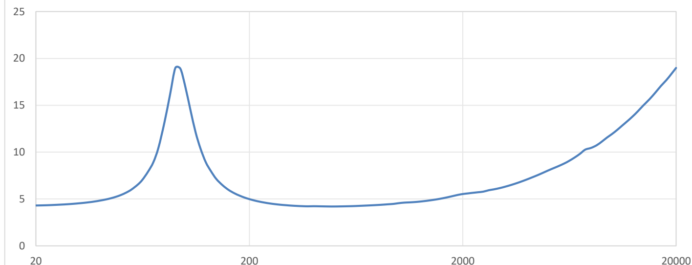
4寸全频-1W/1m
